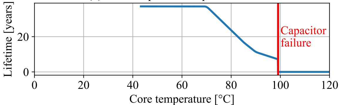
(b) Core temperature impact on lifetime
