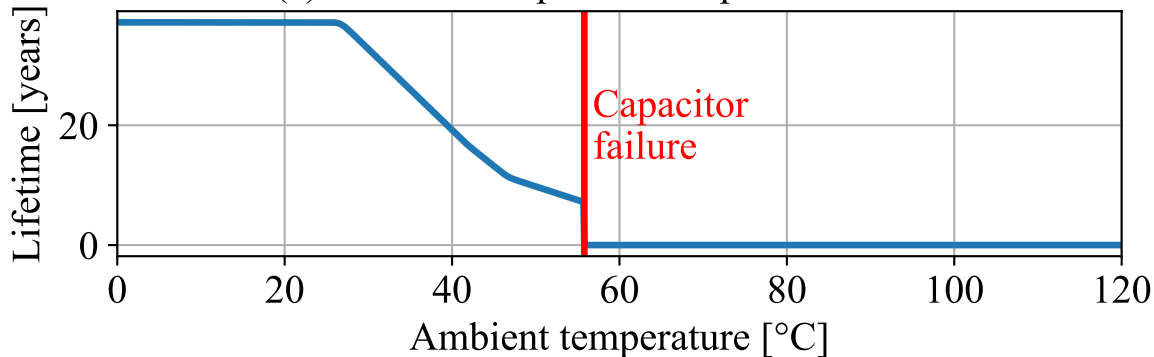
(a) Ambient temperature impact of lifetime
